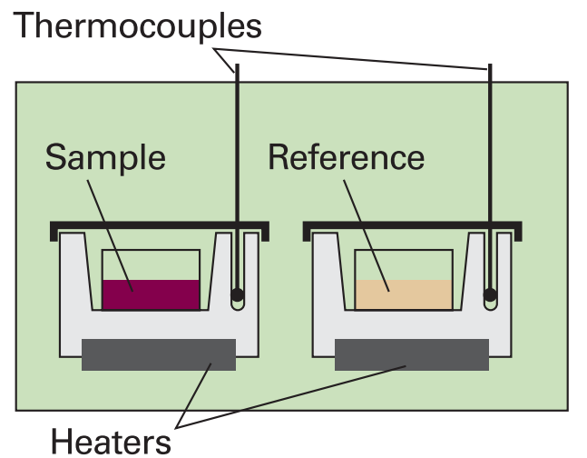
Fig. 2.15 A differential scanning calorimeter. The sample and a reference material are heated in separate but identical metal heat sinks. The output is the difference in power needed to maintain the heat sinks at equal temperatures as the temperature rises.
