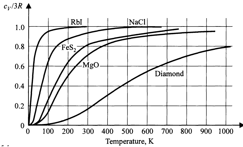
Figure 2: Specific heats of various solids
